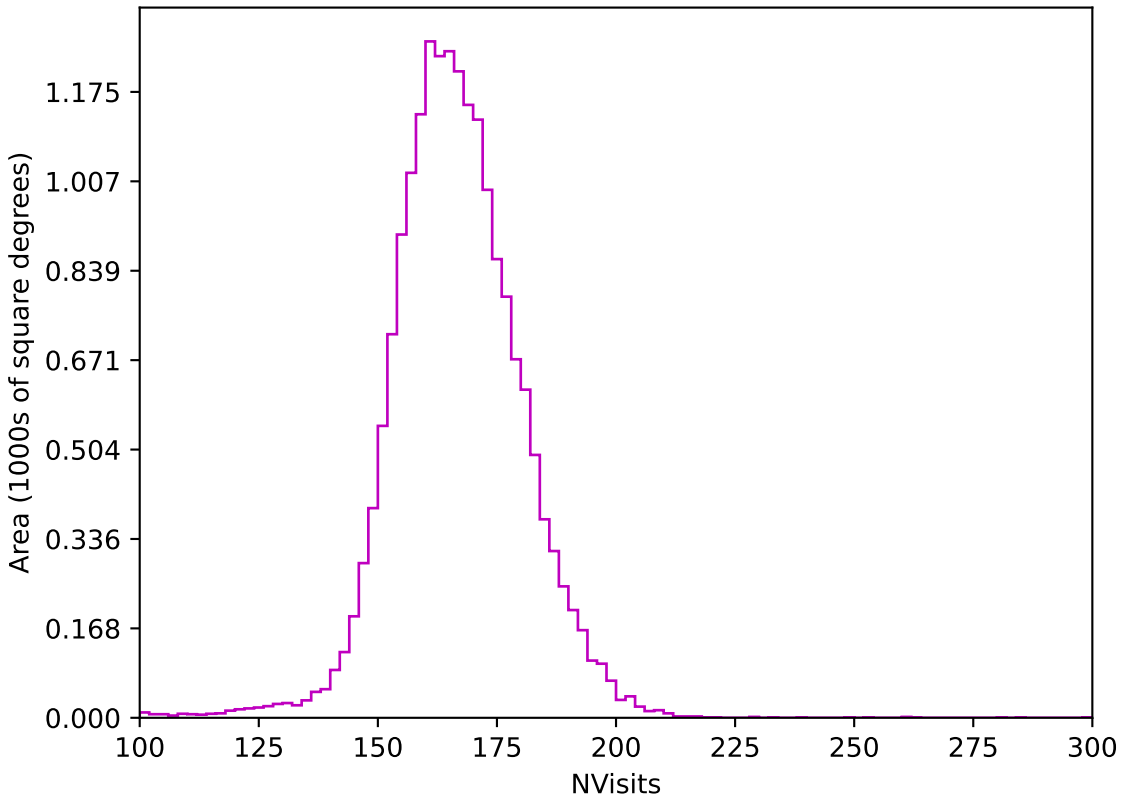
telescope_jerk_v3.5_10yrs WFD z band: NVisits
