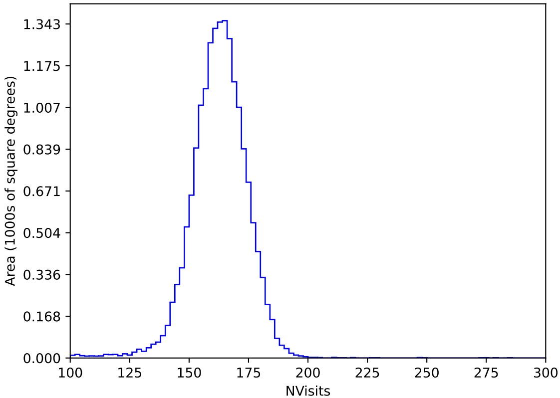
telescope_jerk_v3.5_10yrs WFD y band: NVisits
