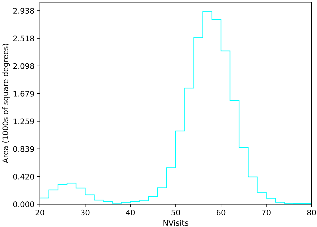
telescope_jerk_v3.5_10yrs WFD u band: NVisits
