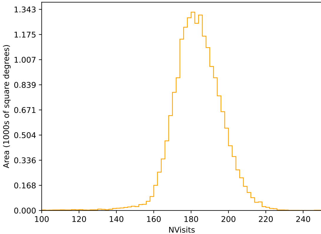
telescope_jerk_v3.5_10yrs WFD r band: NVisits
