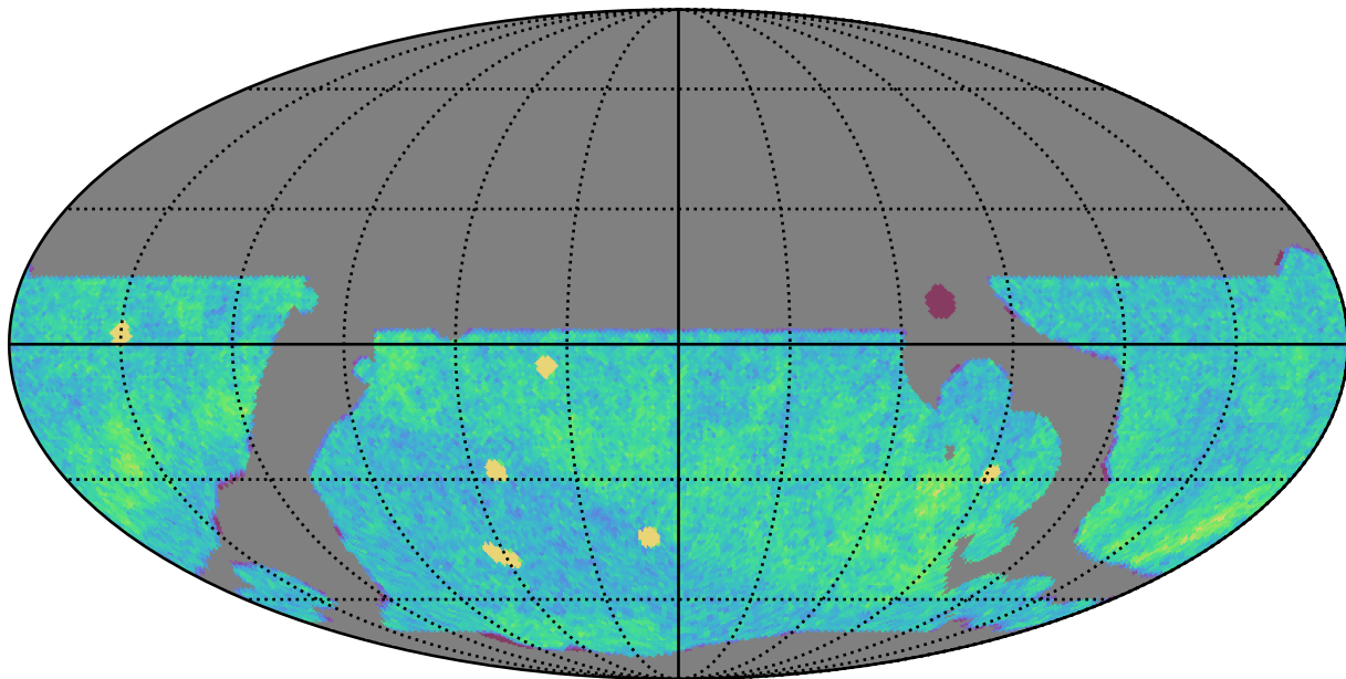
telescope_jerk_v3.5_10yrs WFD i band: NVisits
