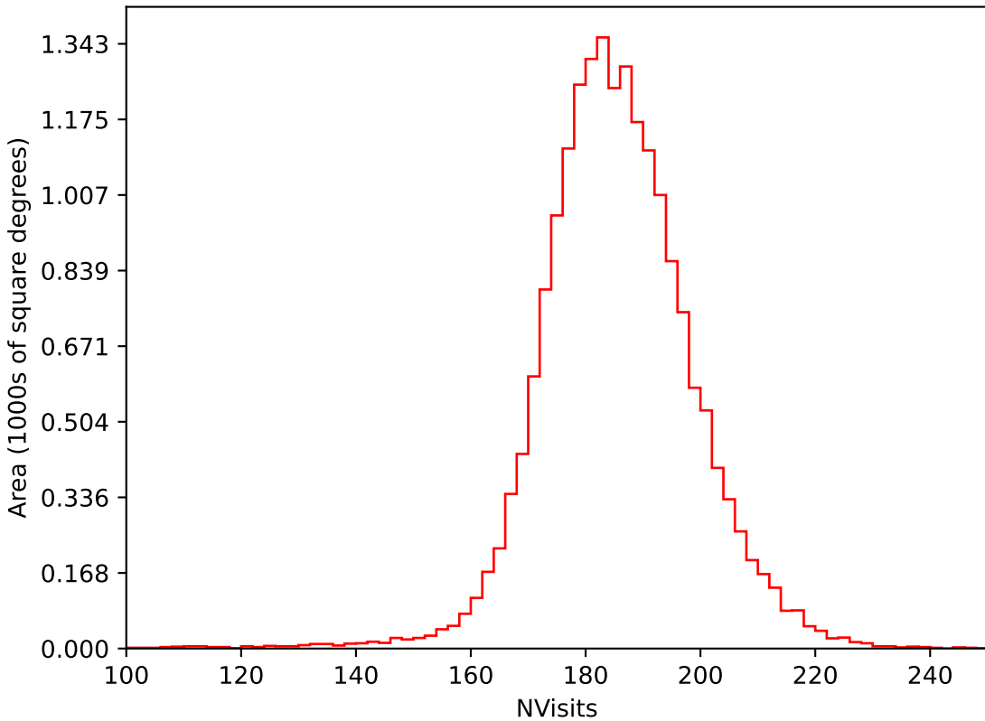
telescope_jerk_v3.5_10yrs WFD i band: NVisits
