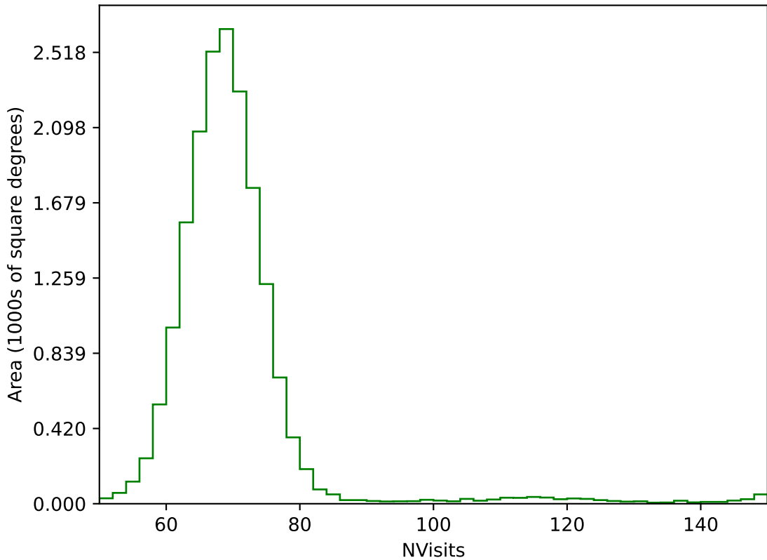
telescope_jerk_v3.5_10yrs WFD g band: NVisits
