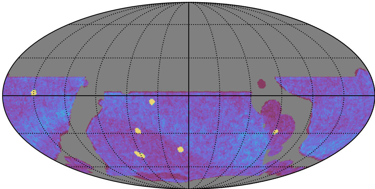
telescope_jerk_v3.5_10yrs WFD all bands: NVisits
