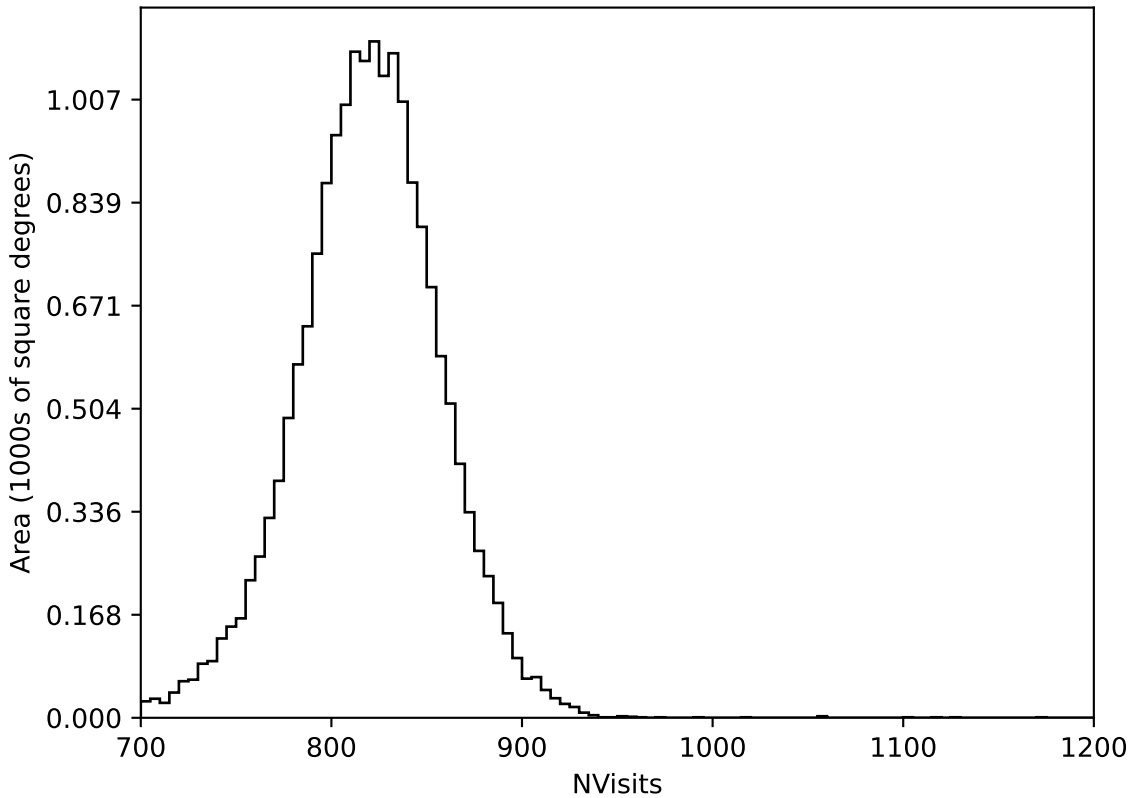
telescope_jerk_v3.5_10yrs WFD all bands: NVisits
