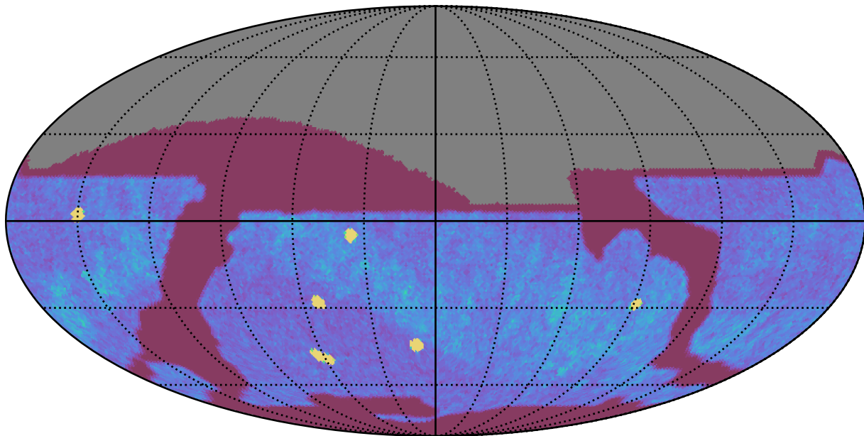
telescope_jerk_v3.5_10yrs All sky z band: NVisits
