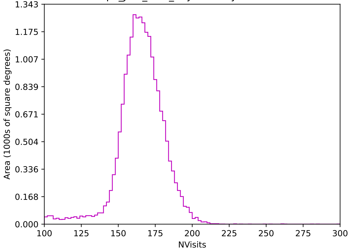
telescope_jerk_v3.5_10yrs All sky z band: NVisits
