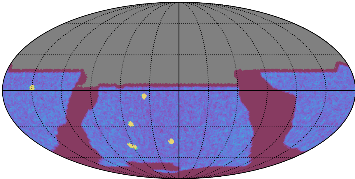
telescope_jerk_v3.5_10yrs All sky y band: NVisits
