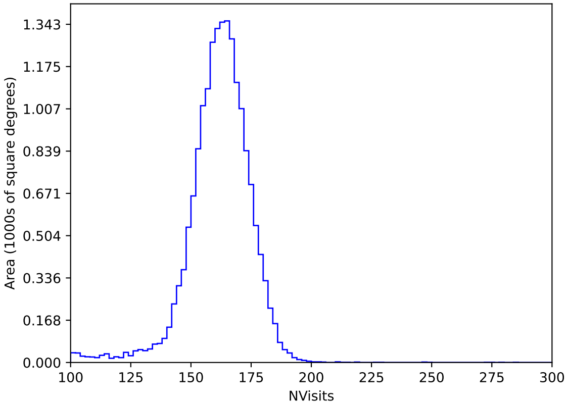
telescope_jerk_v3.5_10yrs All sky y band: NVisits
