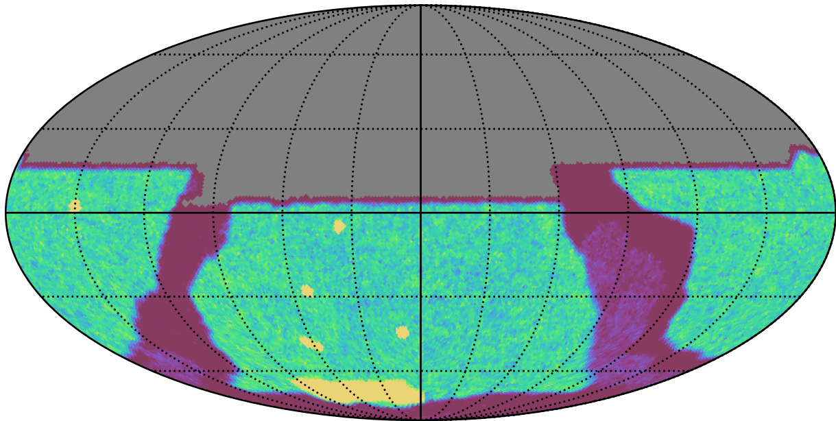
telescope_jerk_v3.5_10yrs All sky u band: NVisits
