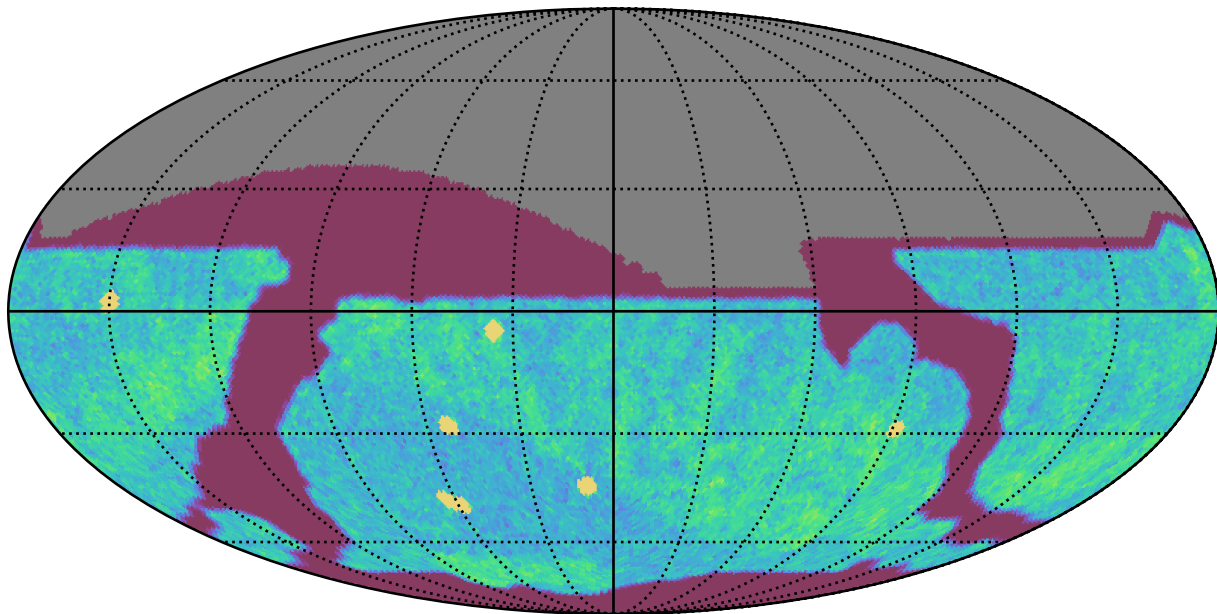
telescope_jerk_v3.5_10yrs All sky r band: NVisits
