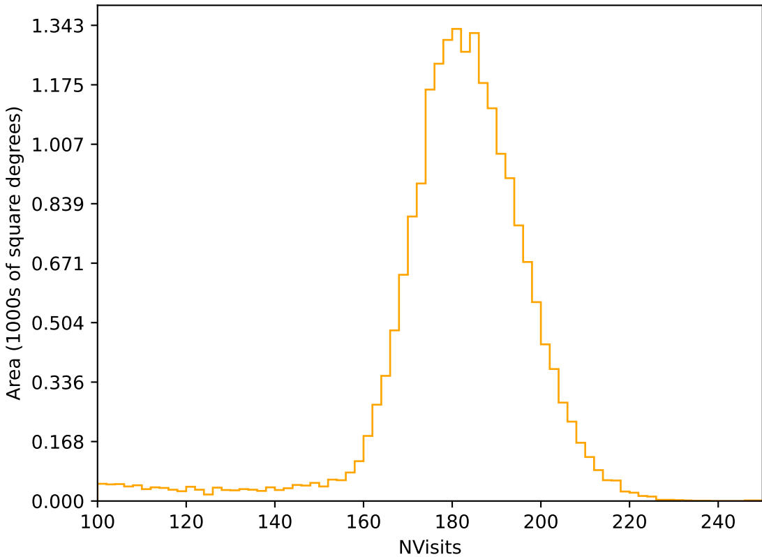
telescope_jerk_v3.5_10yrs All sky r band: NVisits
