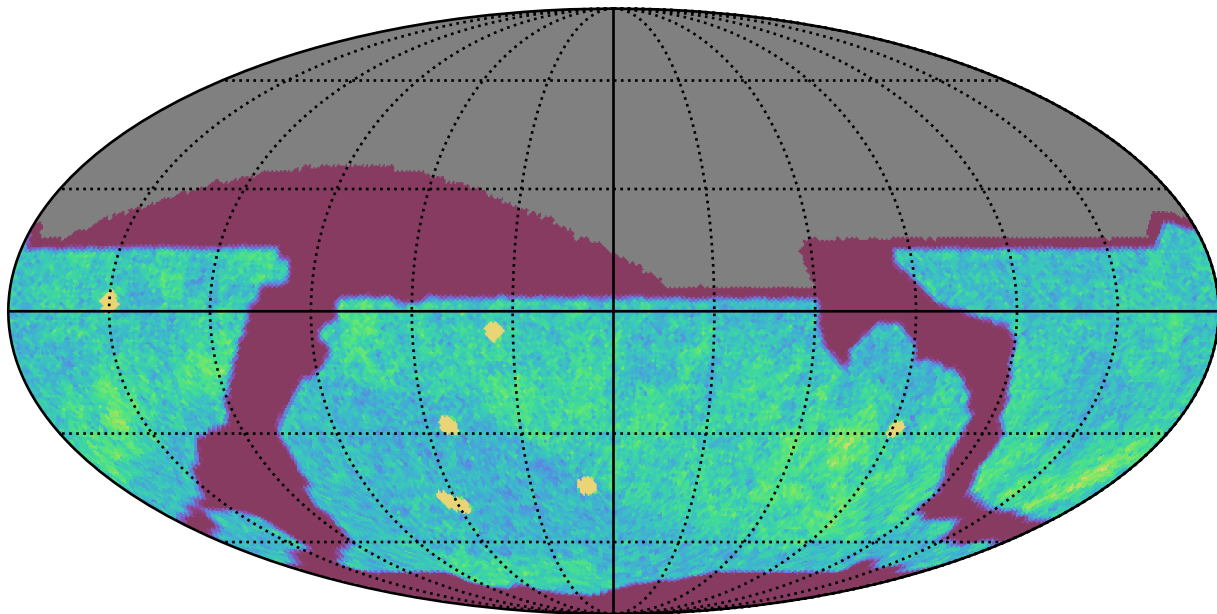
telescope_jerk_v3.5_10yrs All sky i band: NVisits
