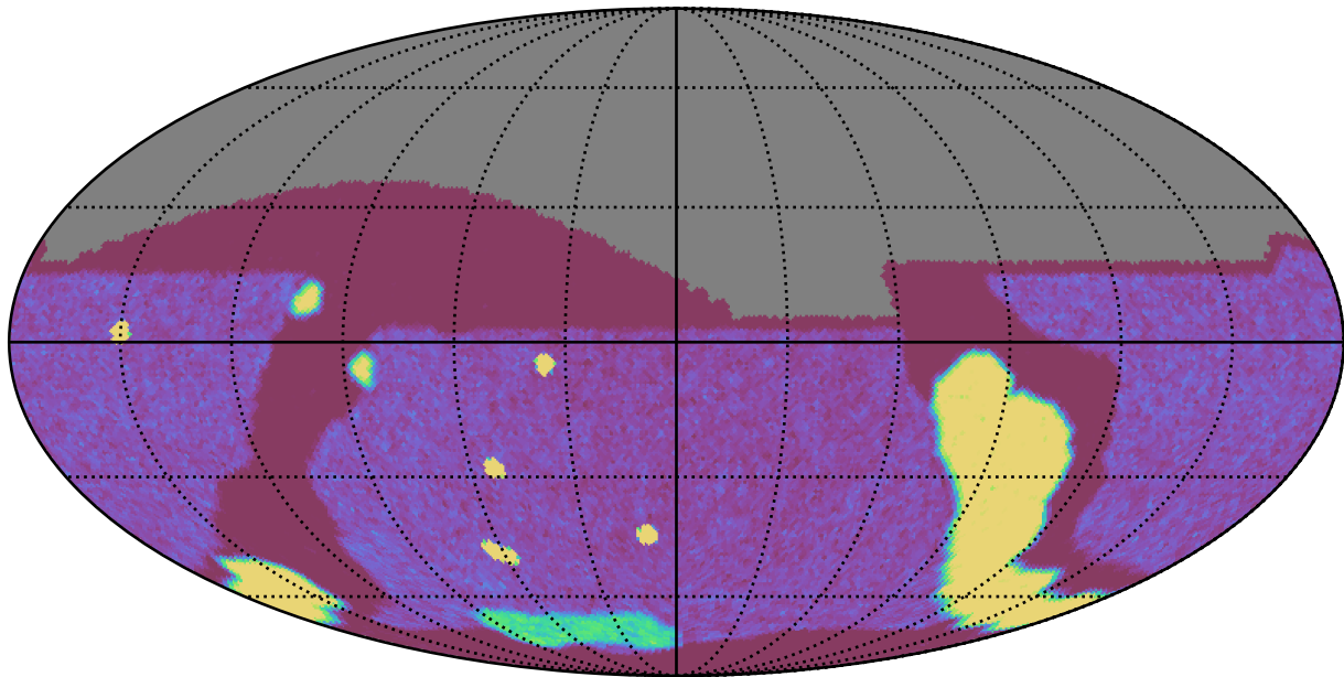
telescope_jerk_v3.5_10yrs All sky g band: NVisits
