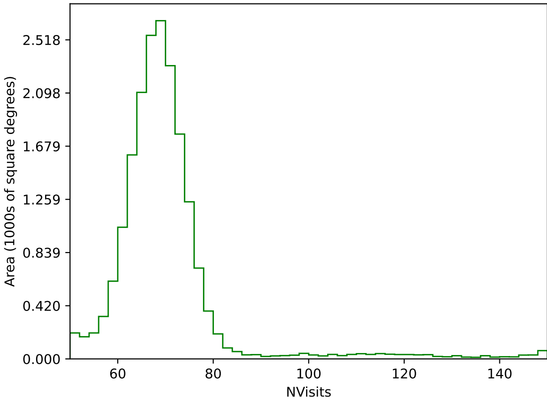
telescope_jerk_v3.5_10yrs All sky g band: NVisits
