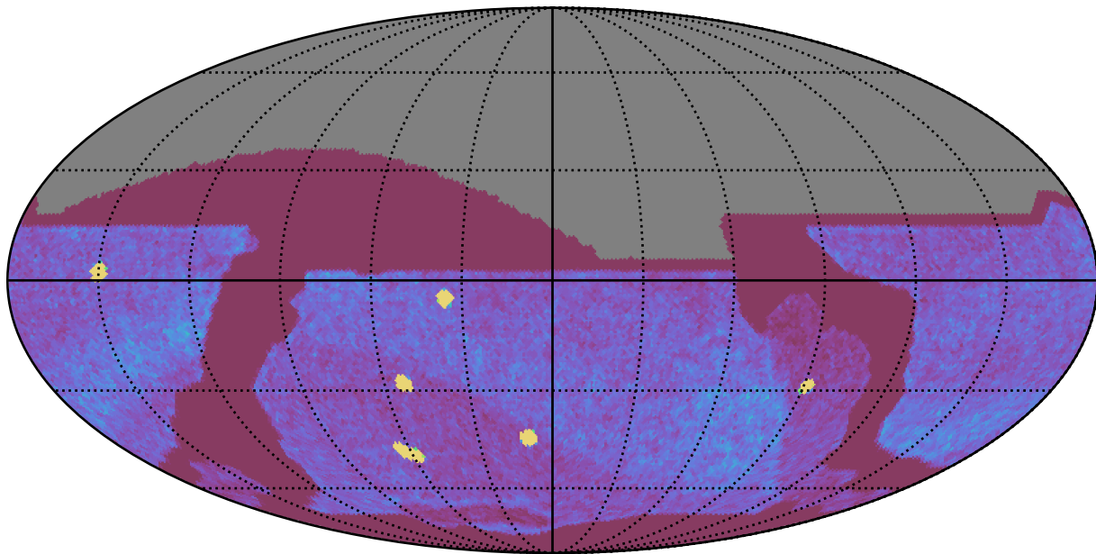
telescope_jerk_v3.5_10yrs All sky all bands: NVisits
