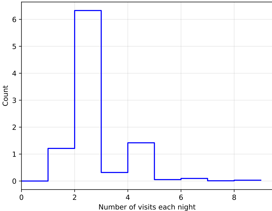
1e6 telescope_jerk_v3.5_10yrs All sky: NVisitsPerNight
