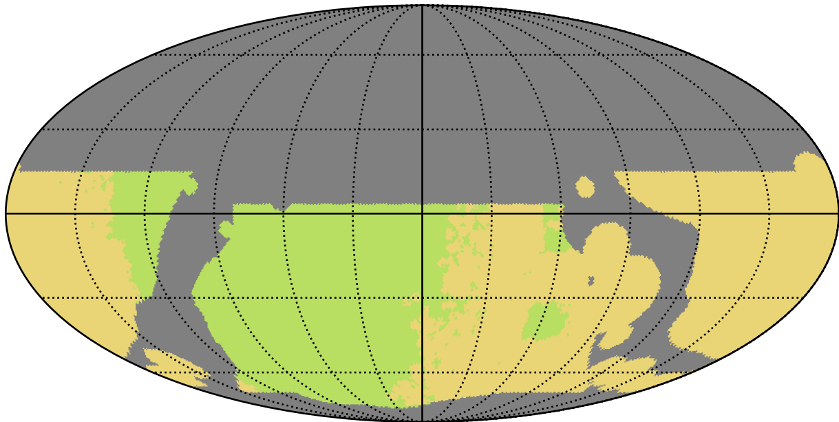
telescope_jerk_v3.5_10yrs WFD all bands: NSeasons
