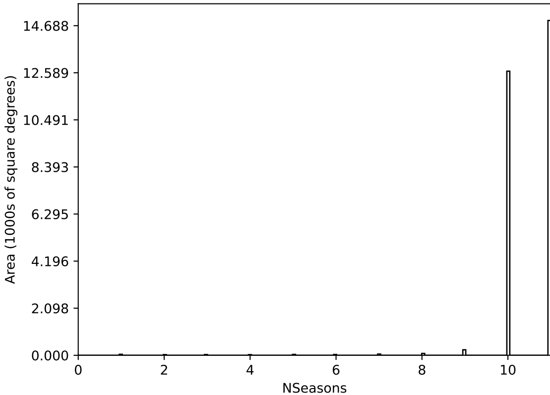
telescope_jerk_v3.5_10yrs All sky all bands: NSeasons
