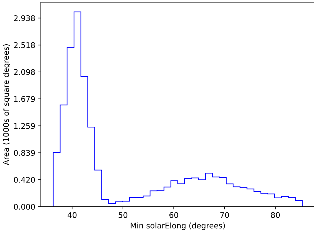
telescope_jerk_v3.5_10yrs WFD z band: Min solarElong
