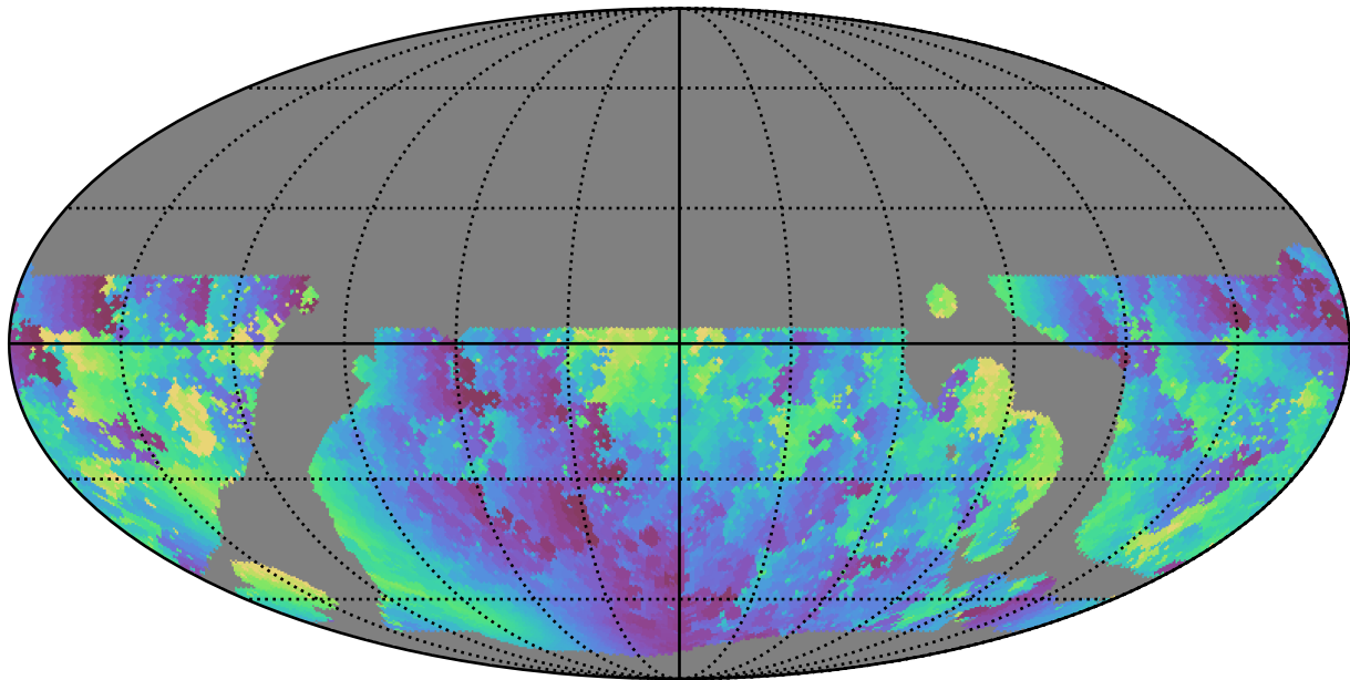
telescope_jerk_v3.5_10yrs WFD u band: Min solarElong
