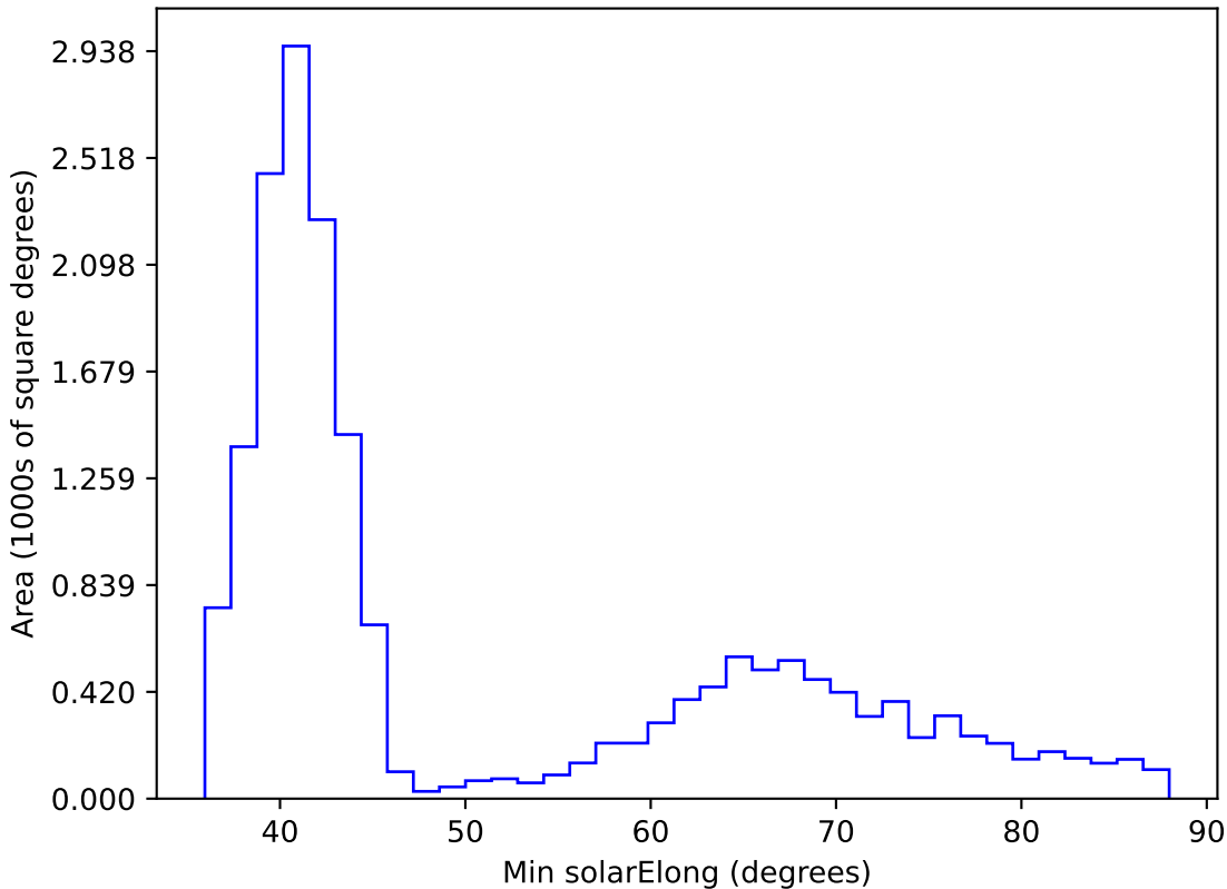
telescope_jerk_v3.5_10yrs WFD r band: Min solarElong
