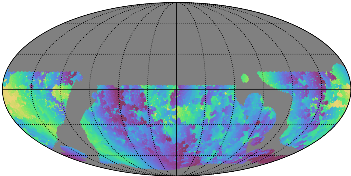
telescope_jerk_v3.5_10yrs WFD g band: Min solarElong
