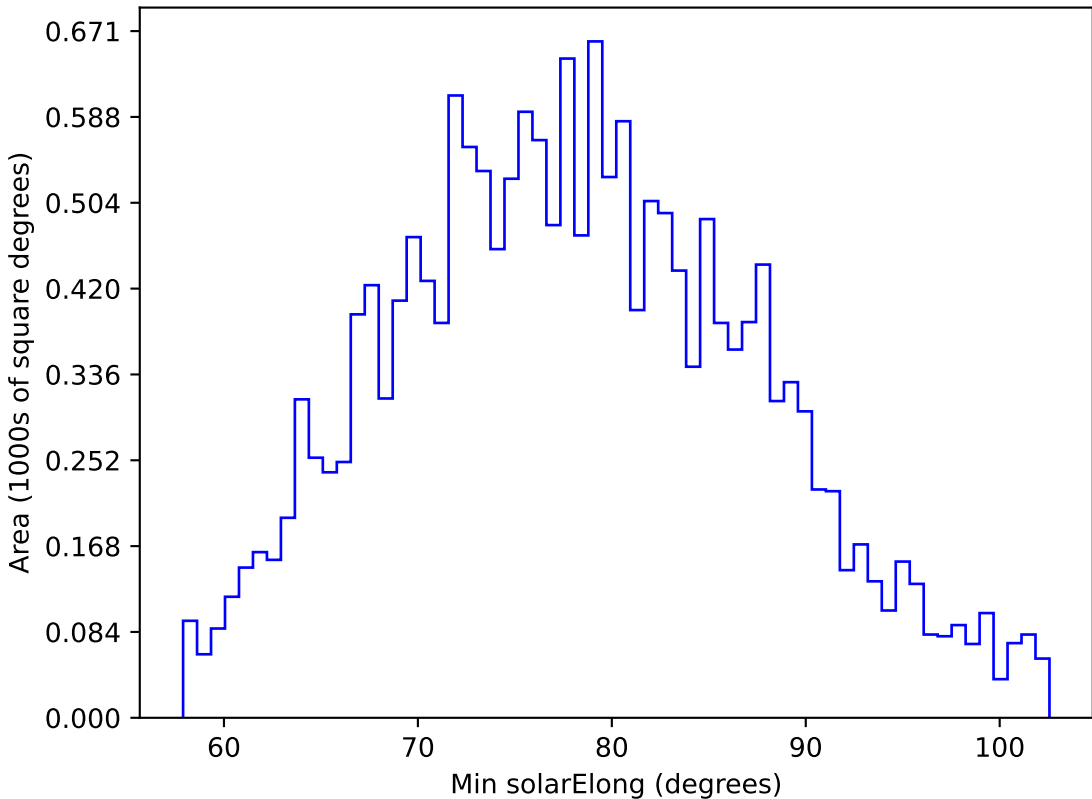
telescope_jerk_v3.5_10yrs WFD g band: Min solarElong
