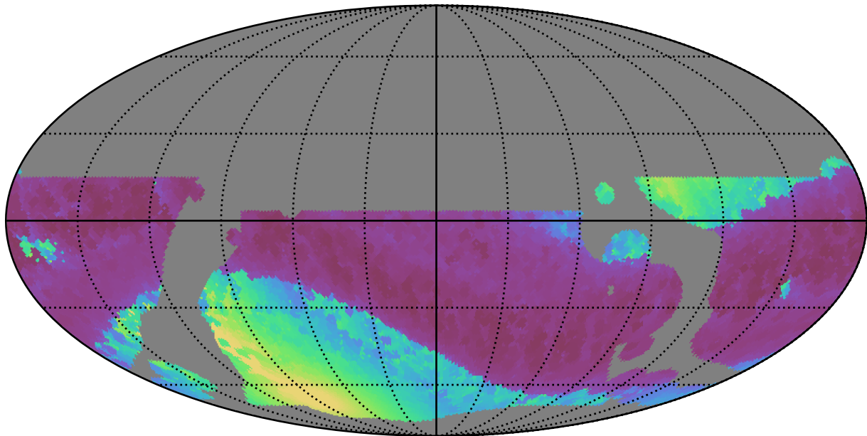
telescope_jerk_v3.5_10yrs WFD all bands: Min solarElong
