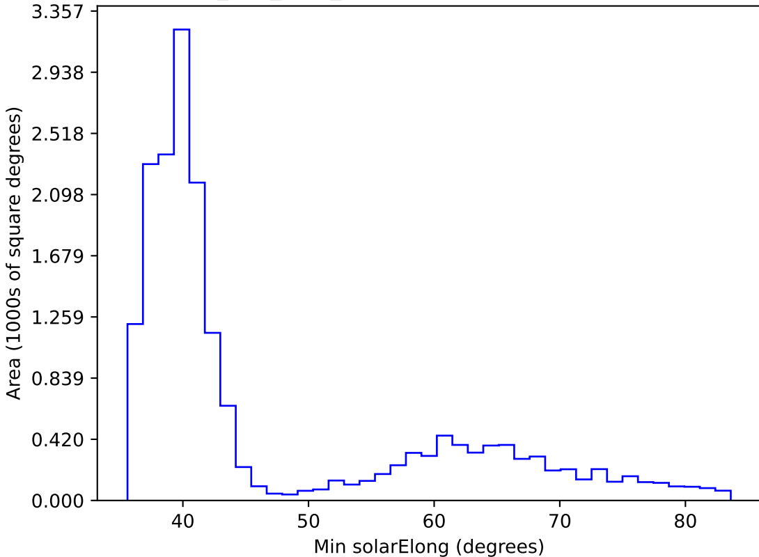
telescope_jerk_v3.5_10yrs WFD all bands: Min solarElong
