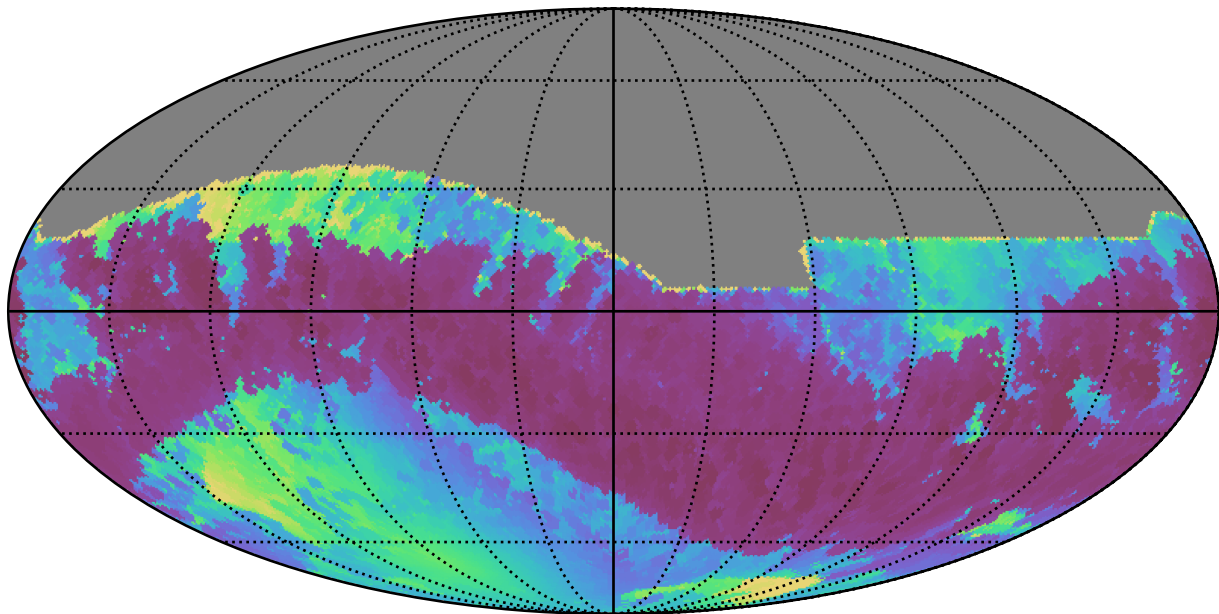
telescope_jerk_v3.5_10yrs All sky z band: Min solarElong
