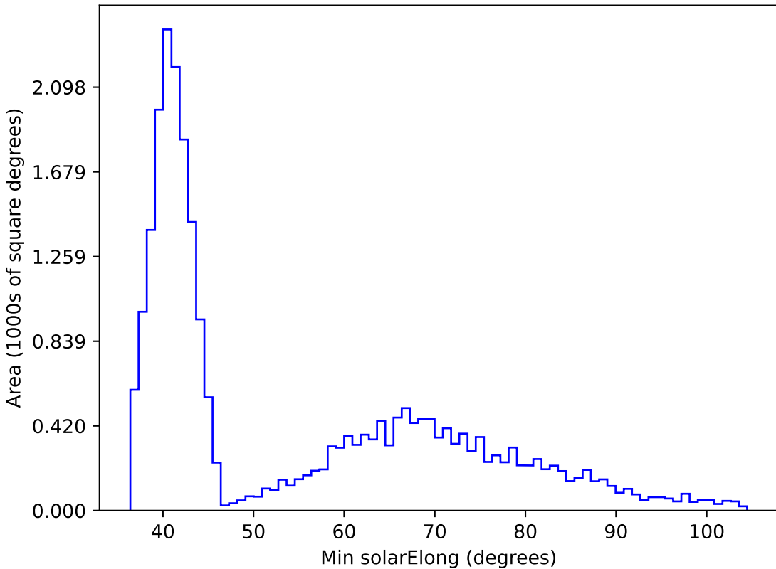
telescope_jerk_v3.5_10yrs All sky z band: Min solarElong
