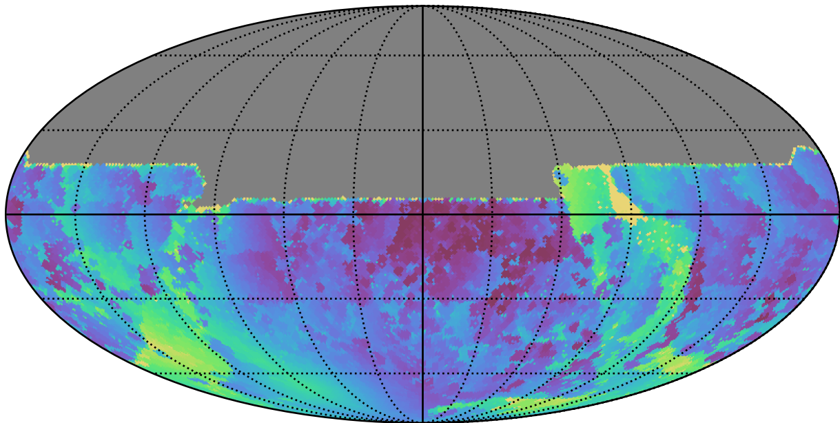
telescope_jerk_v3.5_10yrs All sky y band: Min solarElong
