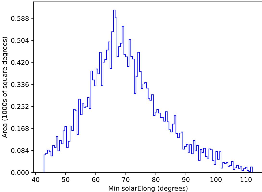
telescope_jerk_v3.5_10yrs All sky y band: Min solarElong
