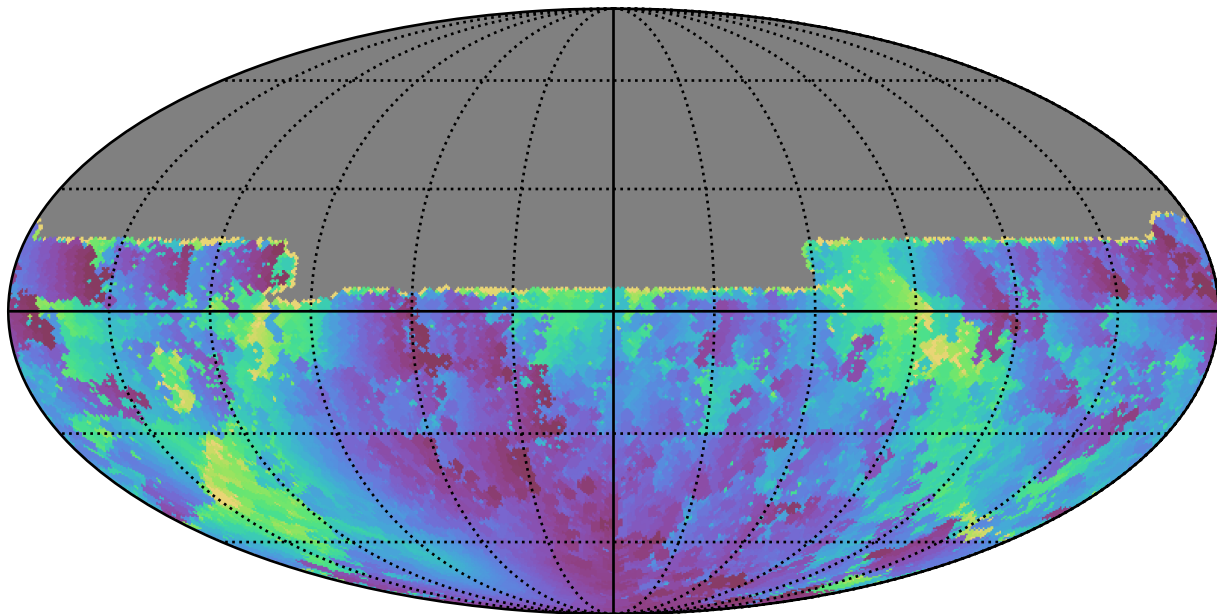
telescope_jerk_v3.5_10yrs All sky u band: Min solarElong
