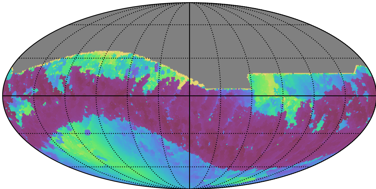
telescope_jerk_v3.5_10yrs All sky r band: Min solarElong
