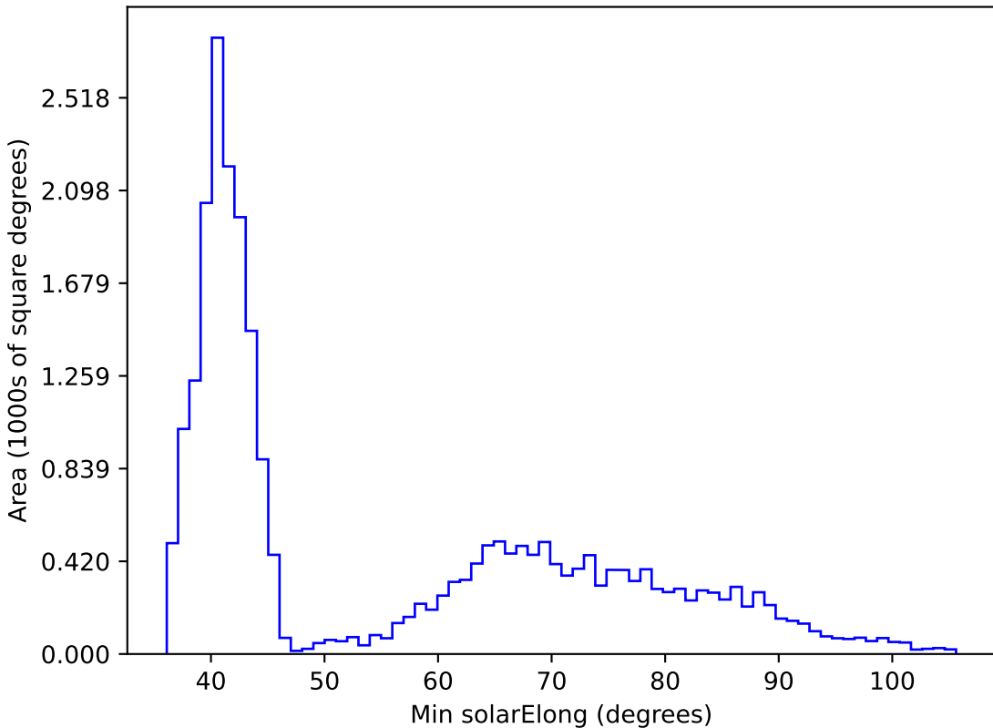
telescope_jerk_v3.5_10yrs All sky r band: Min solarElong
