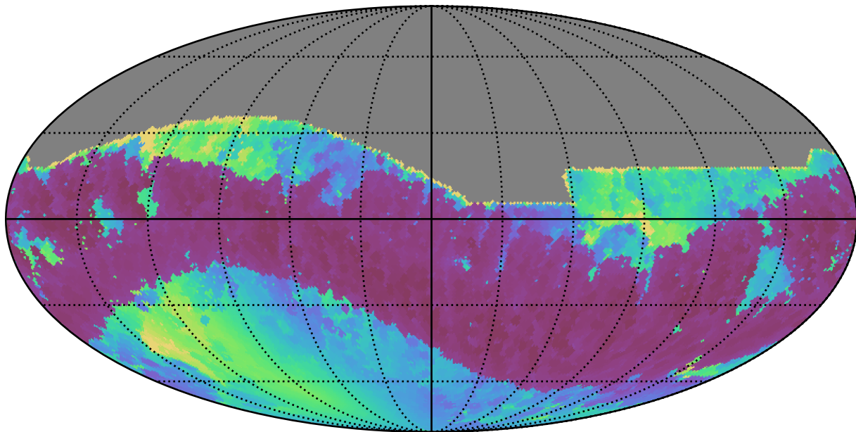
telescope_jerk_v3.5_10yrs All sky i band: Min solarElong
