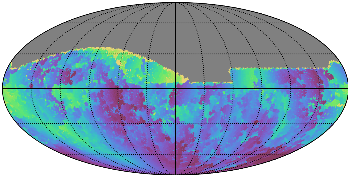
telescope_jerk_v3.5_10yrs All sky g band: Min solarElong
