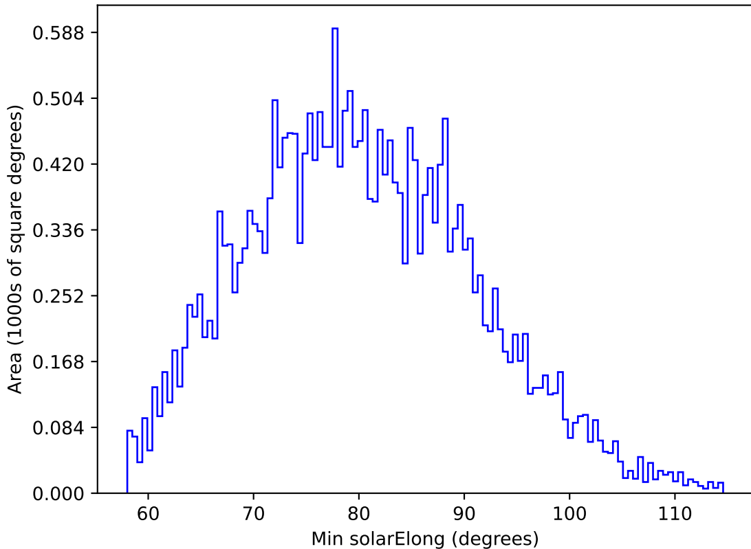
telescope_jerk_v3.5_10yrs All sky g band: Min solarElong
