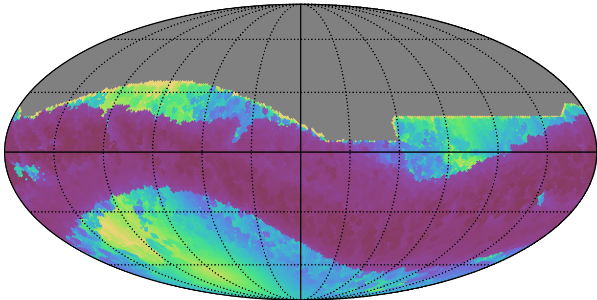
telescope_jerk_v3.5_10yrs All sky all bands: Min solarElong
