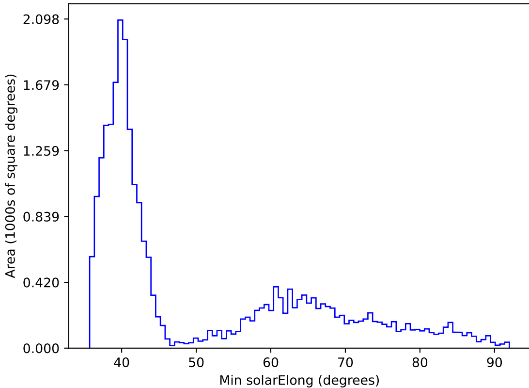
telescope_jerk_v3.5_10yrs All sky all bands: Min solarElong
