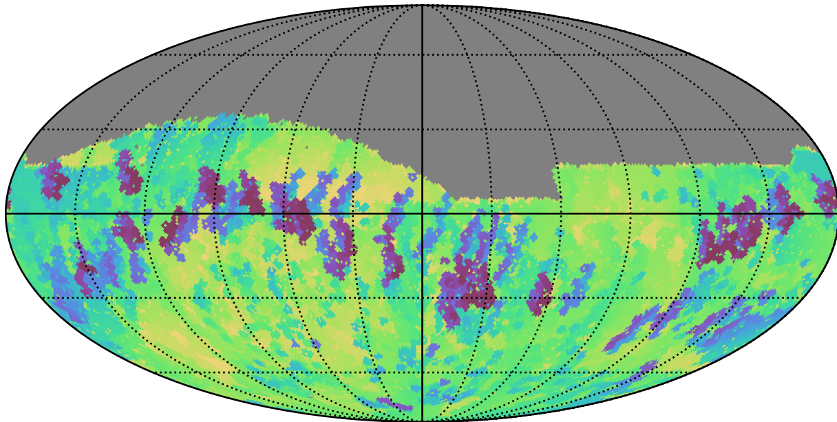
telescope_jerk_v3.5_10yrs Yr 1 z band: Min skyBrightness
