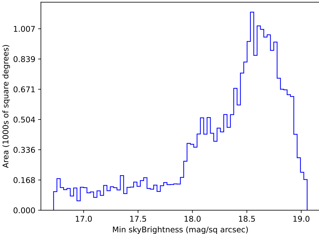
telescope_jerk_v3.5_10yrs Yr 1 z band: Min skyBrightness
