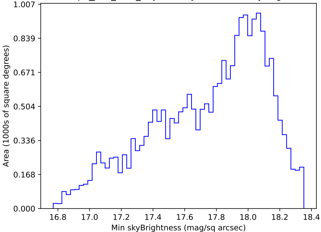
telescope_jerk_v3.5_10yrs Yr 1 y band: Min skyBrightness
