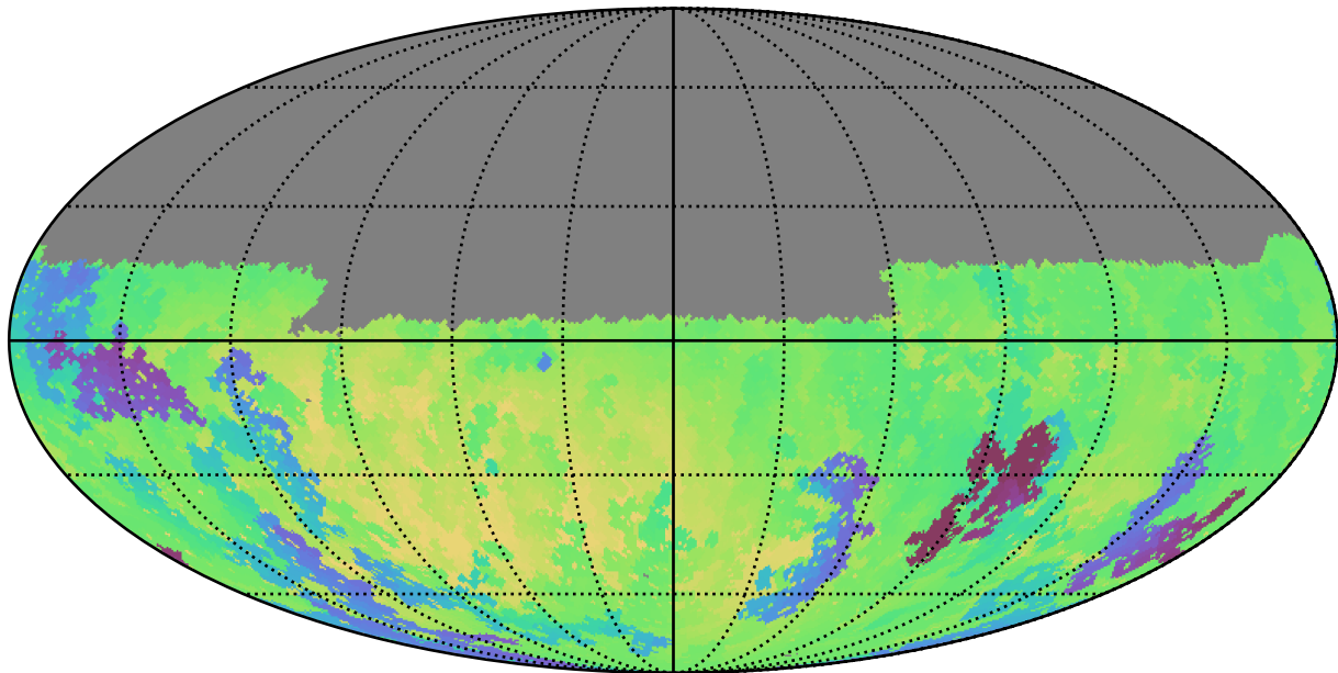
telescope_jerk_v3.5_10yrs Yr1 u band: Min skyBrightness
