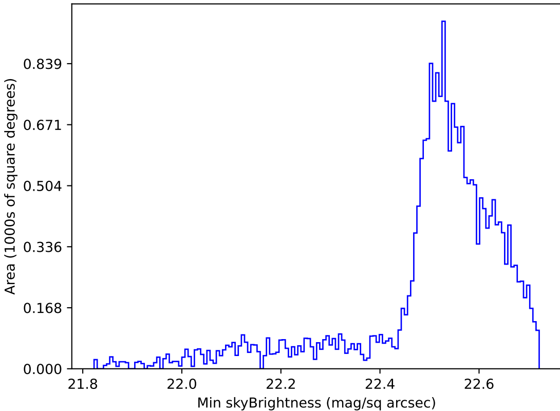
telescope_jerk_v3.5_10yrs Yr 1 u band: Min skyBrightness
