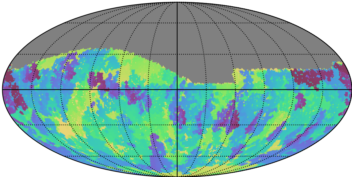
telescope_jerk_v3.5_10yrs Yr 1 r band: Min skyBrightness
