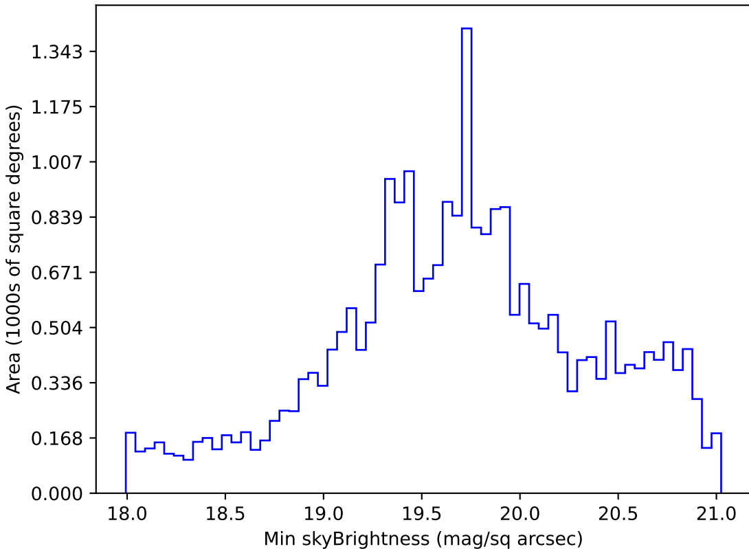
telescope_jerk_v3.5_10yrs Yr 1 r band: Min skyBrightness
