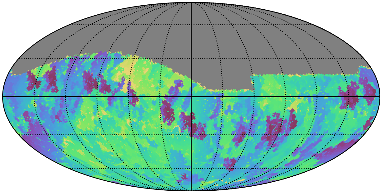
telescope_jerk_v3.5_10yrs Yr 1 i band: Min skyBrightness
